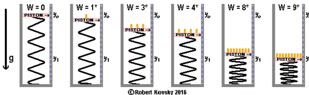
Hooke's Law -- spring force in equipose with gravitational force
